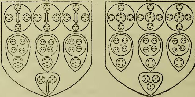
Indium
